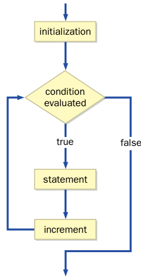
figure 3.9 The logic of a for loop
