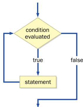
figure 3.8 The logic of a while loop
